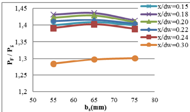
Fig. 23 Effect of ( b_s ) on the Failure Load ( t_s = 3.0 mm & a/d_w=3.0 )
