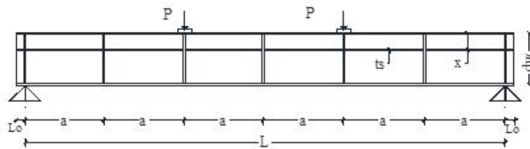
(b) Studied beams for a/d w =1.5
