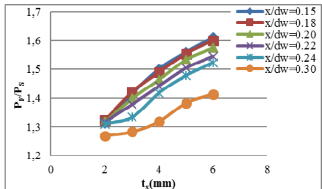
Fig. 20 Effect of ( t_s ) on the Failure Load ( a/d_w=1.5 & b_s=75 mm)
