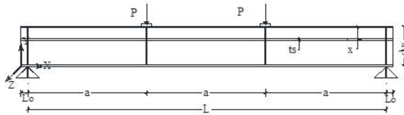
(a) Studied beams for a/d w =3
