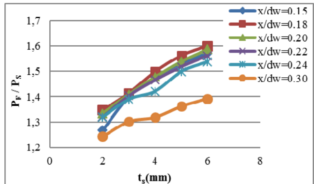
Fig. 19 Effect of ( t_s ) on the Failure Load ( a/d_w=3.0 & b_s=75 mm)
