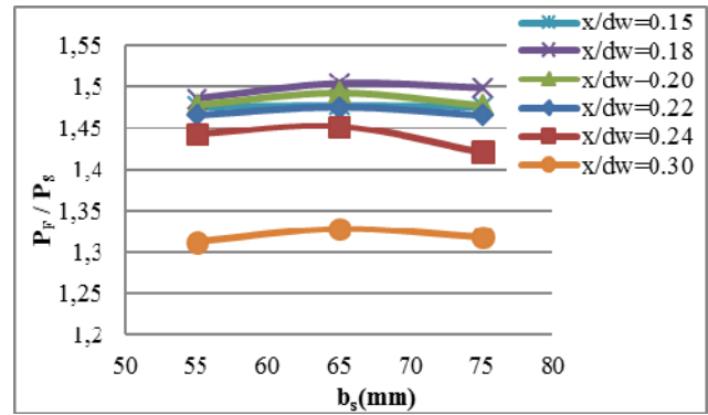
Fig. 24 Effect of ( b_s ) on the Failure Load ( t_s = 4.0 mm & a/d_w=3.0 )
