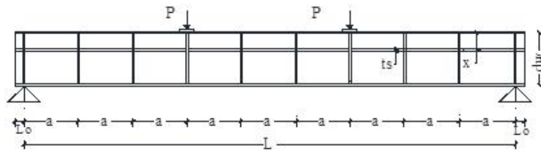
(c) Studied beams for a/d w =1
