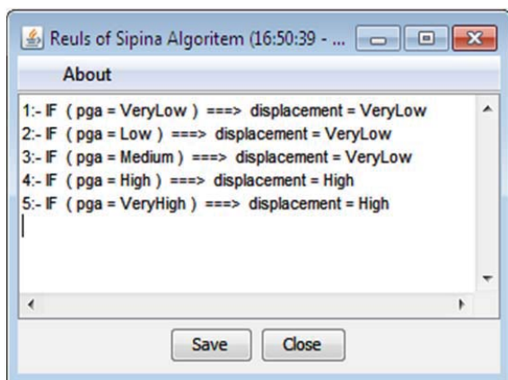
Fig. 7 Generated rules
