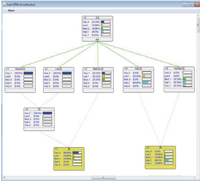
Fig. 2 Generated graph
