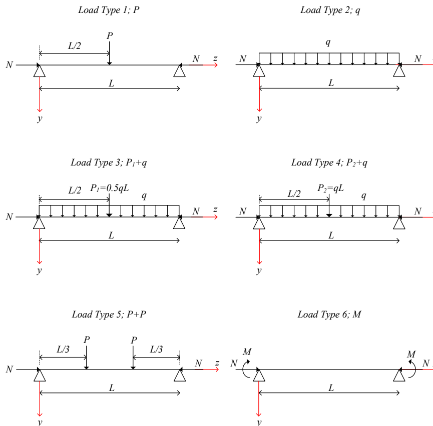
Fig. 3 Load types
