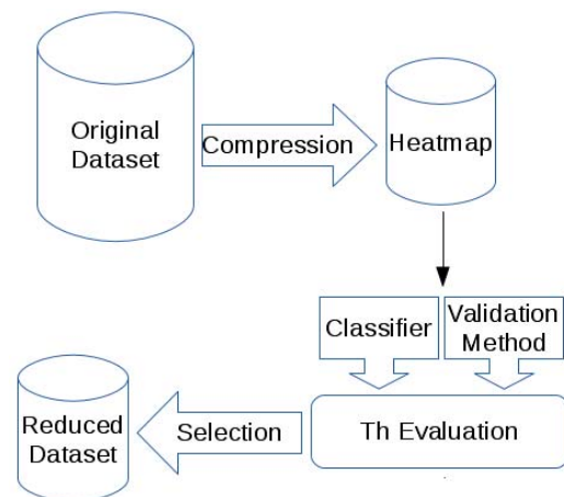
Fig. 1 Proposed architecture for optimal threshold selection
