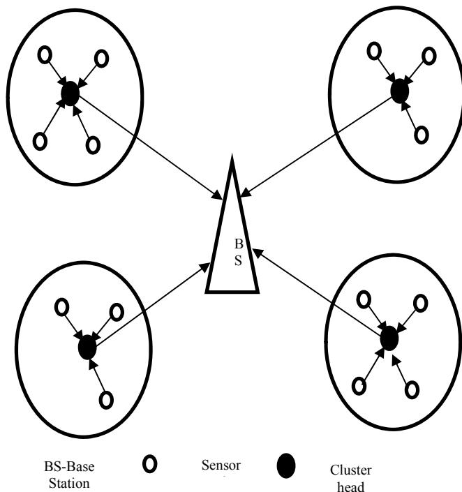
Fig. 3 LEACH
