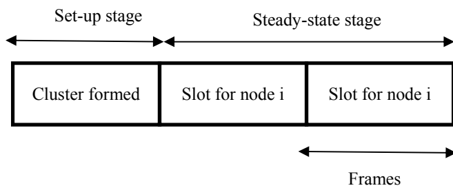
Fig. 2 LEACH Stages
