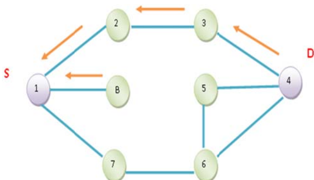
Fig. 2 RRES Replying
