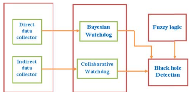
Fig. 6 Architecture of collaborative watchdog with fuzzy logic
