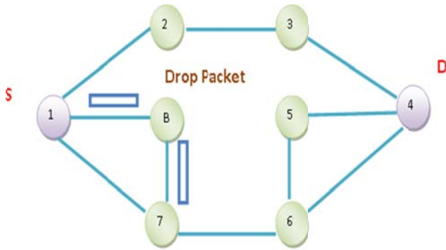
Fig. 3 Blackhole Attack
