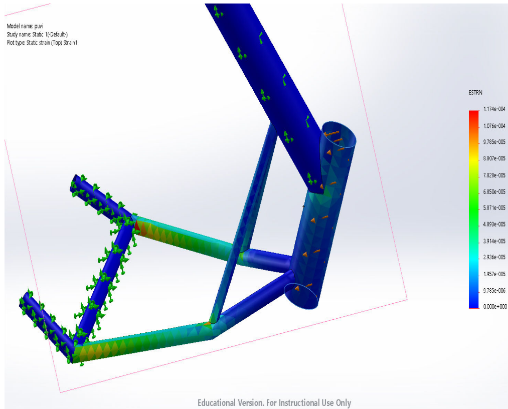
Fig. 7 Analysis of strain
