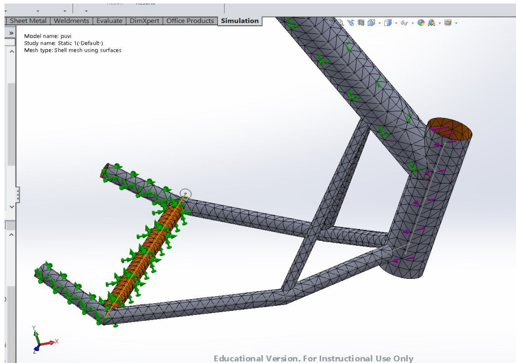
Fig. 6 Shell mesh using surfaces
