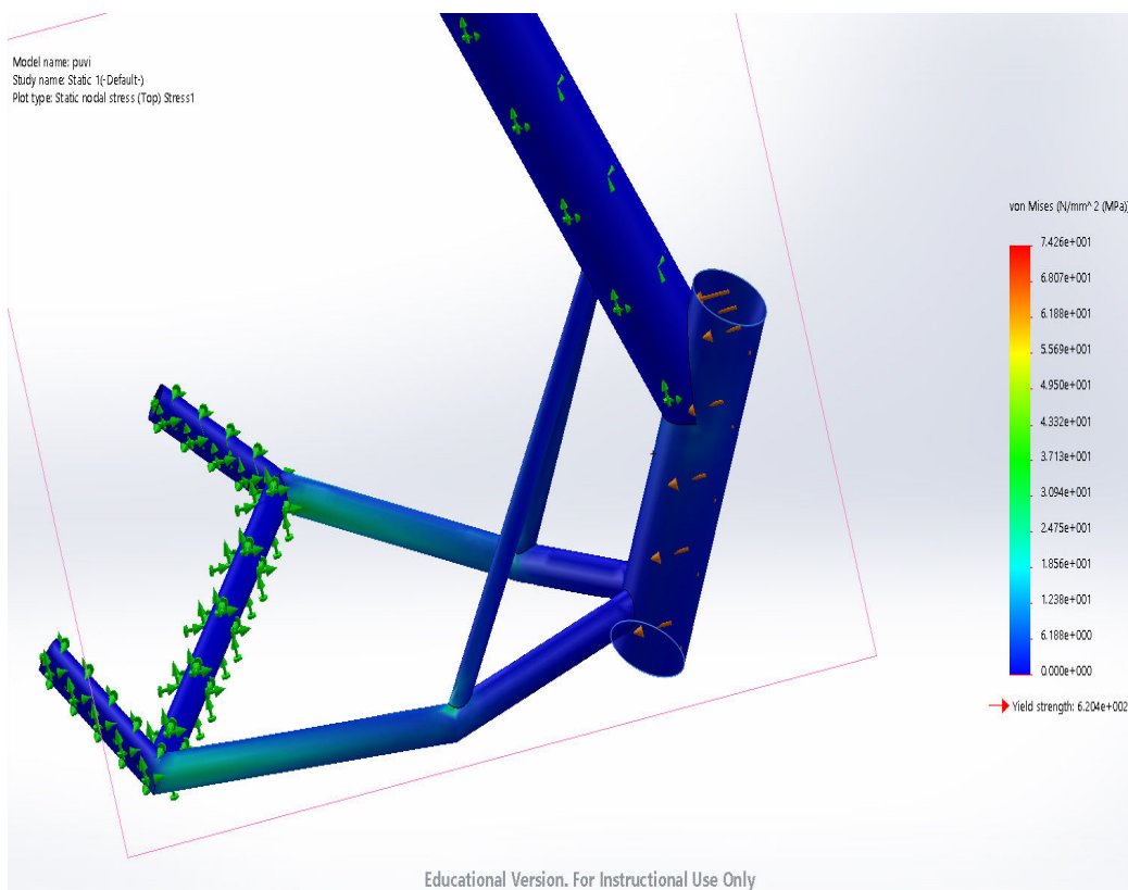
Fig. 8 Analysis of stress
