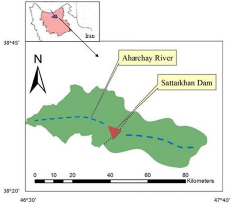
Fig. 1 Aharchay watershed Location (adapted from [7])
