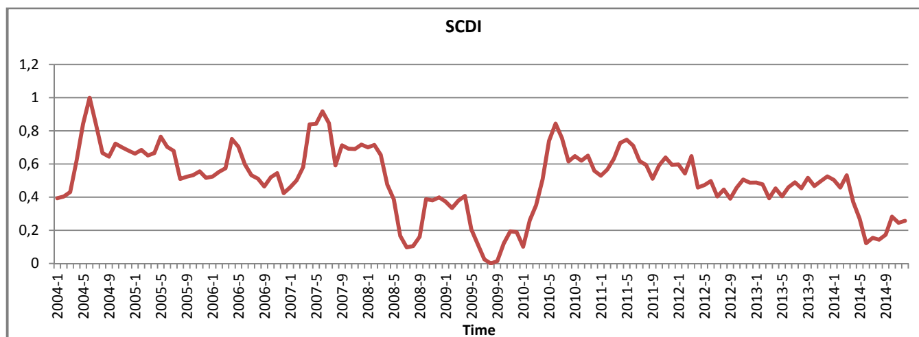
Fig. 4 Standardized CDI variation
