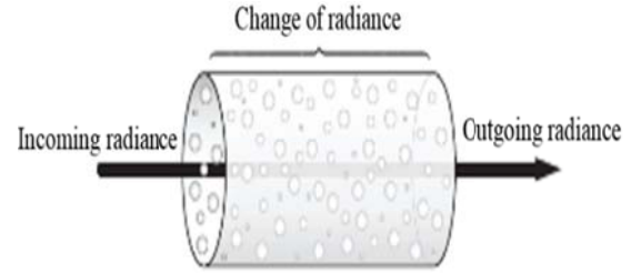
Fig. 2 The participating media as a collection of microscopic scattering particles
