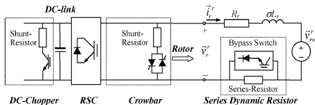
Fig. 6 The crowbar with series dynamic resistance
