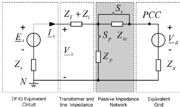
Fig. 12 DFIG with series passive-impedance network
