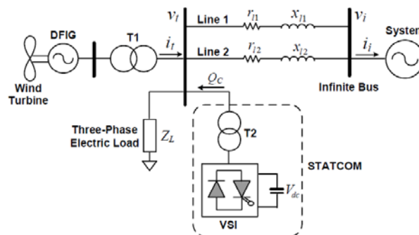
Fig. 7 Applying STATCOM to DFIG
