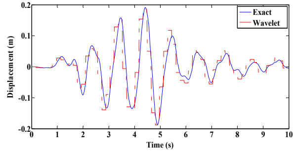
Fig. 2 Roof displacement derived by Haar wavelet compared with exact ones for first shear frame
