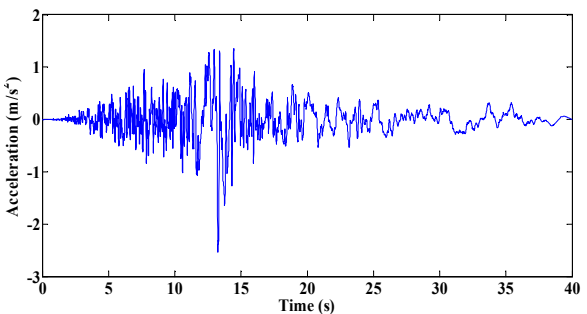
Fig. 4 Acceleration history of Superstition hill
