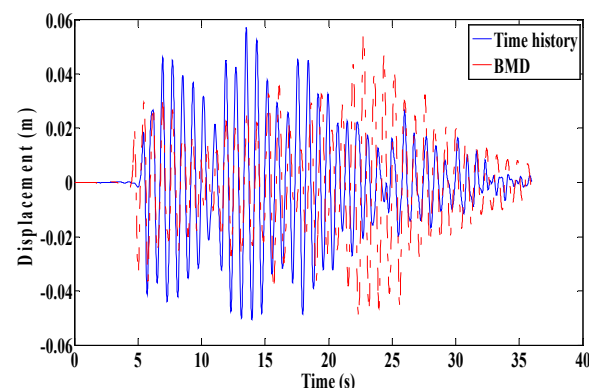
Fig. 7 Roof displacement derived by BMD compared with exact ones for third shear frame, under Artificial quake
