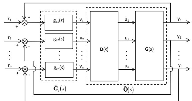
Fig. 1 Block diagram of a decoupling control system
