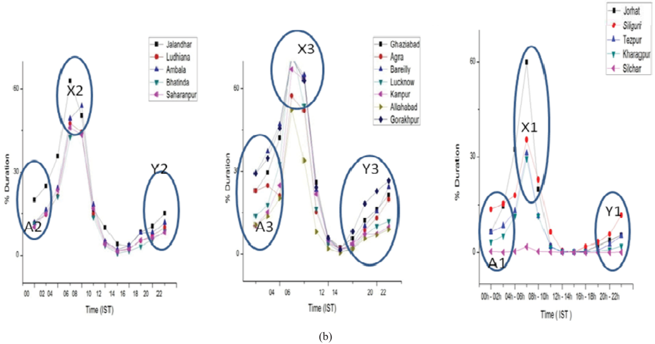
Fig. 12 (a) Diurnal Variability(Jan), (b) Diurnal Variability (Dec)
