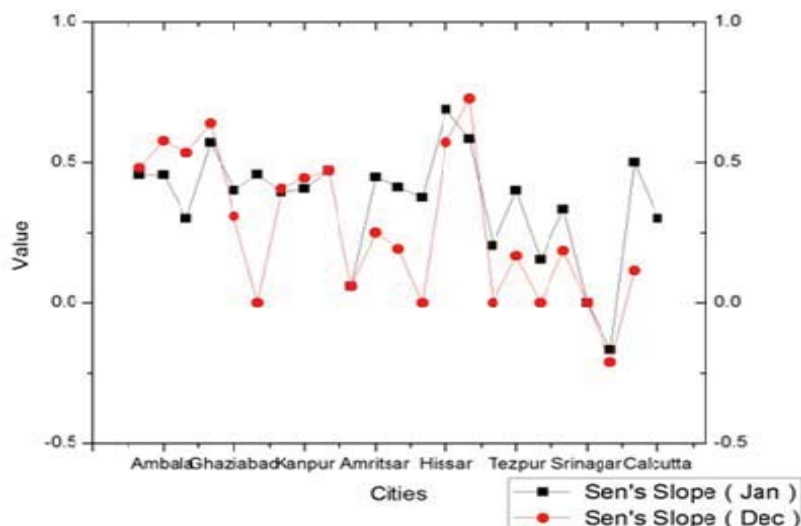
Fig. 9 Theil and Sen's Slope
