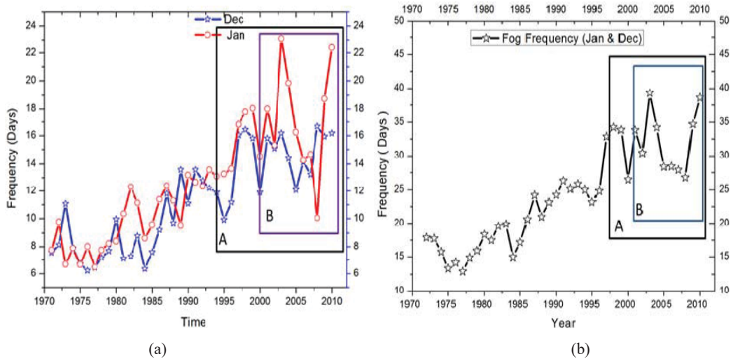
Fig. 5 (a) Time series Analysis (Dec & Jan), (b) Time series Analysis (winter season)
