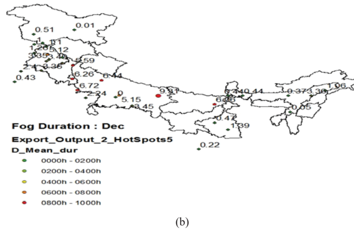
Fig. 13 (a) Average Daily Persistence (January), (b) Average Daily Persistence (December)
