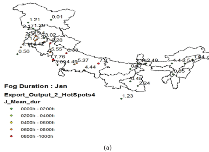
Fig. 12 (a) Diurnal Variability(Jan), (b) Diurnal Variability (Dec)
