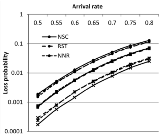
Fig. 6 Comparison of the loss probability (S=1, SFC=15)
