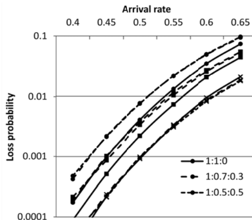
Fig. 8 Comparison of the loss probability (S=1, SFC=20)
