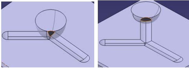
Fig. 3 After completing vertical cutting pass of Y shape on the 1 st cutting layer, fabrication of rightward offset cutting of the 3 rd cutting pass on the 1 st cutting layer was simulated
