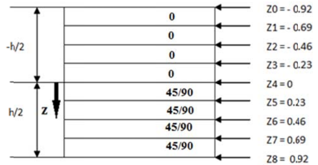
Fig. 5 Schematic architecture of the used materials
