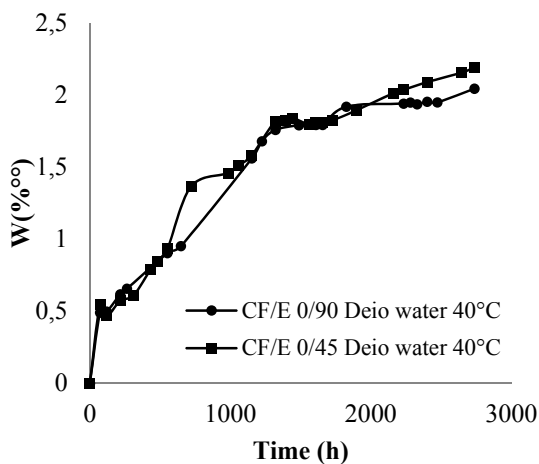
Fig. 2 Kinetic Absorption of Carbone fiber/Epoxy in deionized water at 40°C
