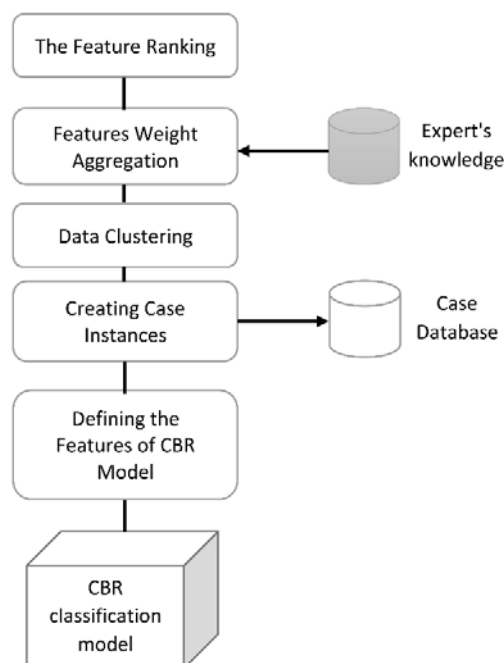
Fig. 2 The concept of classification process
