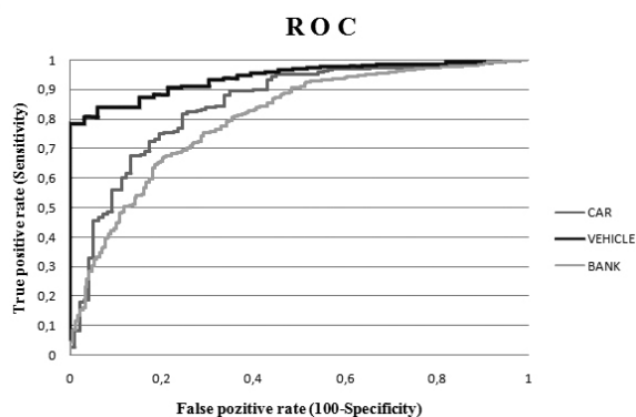
Fig. 3 ROC curves
