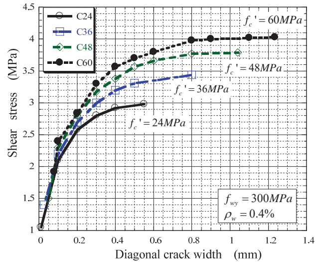
Fig. 6 Effect of compressive strength of concrete
