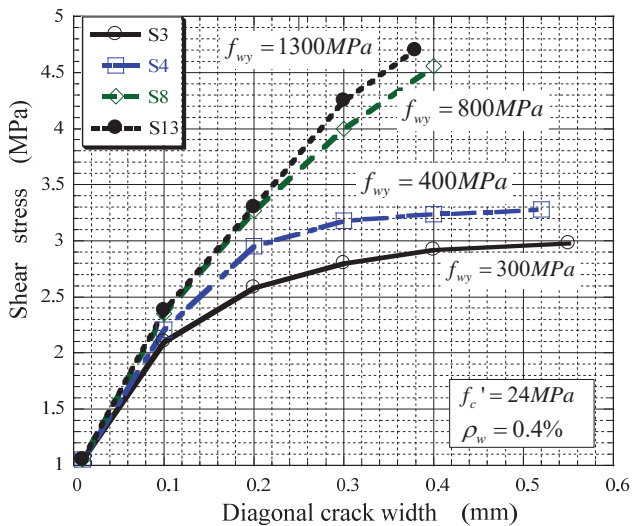
Fig. 5 Effect of yield strength of shear reinforcement
