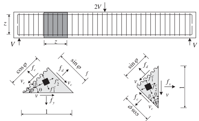
Fig. 1 A compatibility aided truss model
