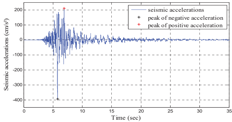
Fig. 4 Example of accelerogram (KeddaraDam)
