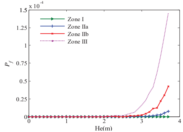
Fig.10 Failure mode by crushing concrete
