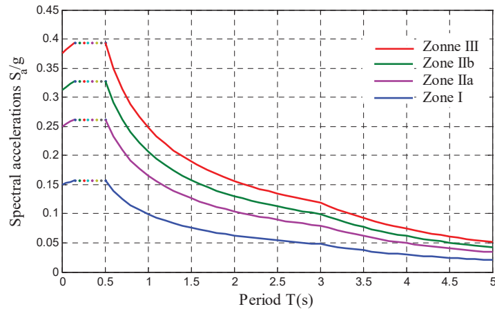
Fig. 3 Response spectra
