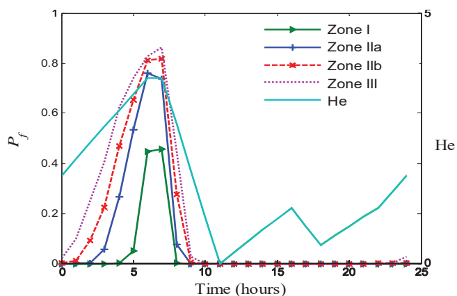
Fig. 17 Failure mode by sloshing
