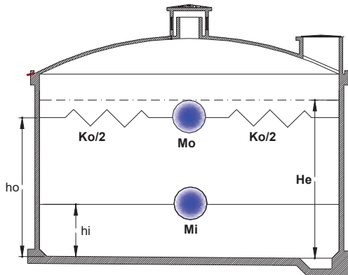
Fig. 1 Equivalent mechanical system
