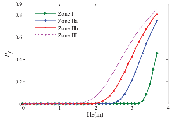
Fig. 12 Failure mode by sloshing
