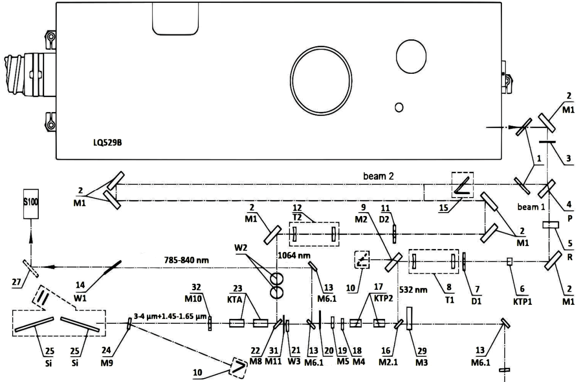
Fig. 1 Optical diagram of the laser system
