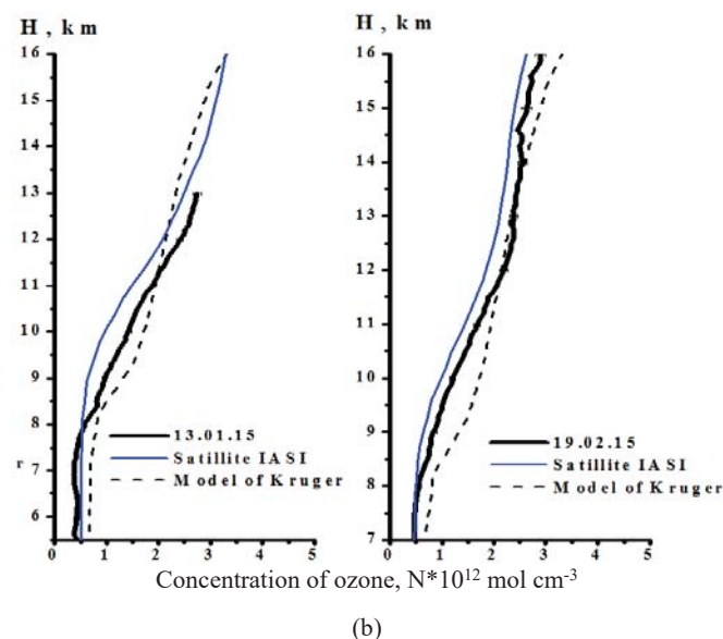
Fig. 2 Retrieved vertical profiles of ozone concentration at wavelengths (299, 341) nm (a) November 2014, (b) January-February 2015) compares them with Krueger midlatitude model and IASI satellite data
