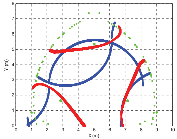
Fig. 15 Singularity loci of actuation2
