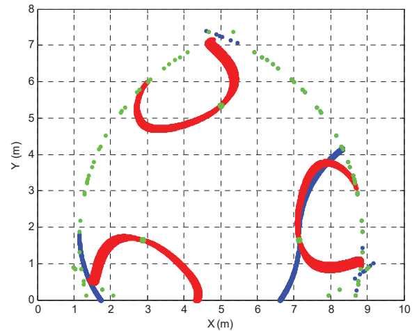
Fig. 9 Singularity loci for actuation 4
