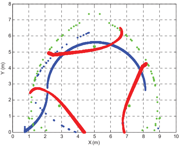
Fig. 18 Singularity loci of actuation 5
