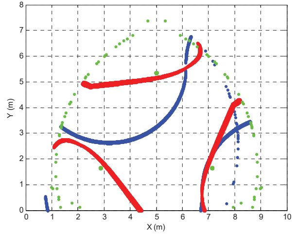
Fig. 19 Singularity loci of actuation 6
