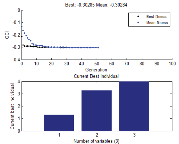
Fig. 22 Convergence of GCI for actuation 1
