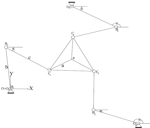
Fig. 1 3RRR parallel manipulator
