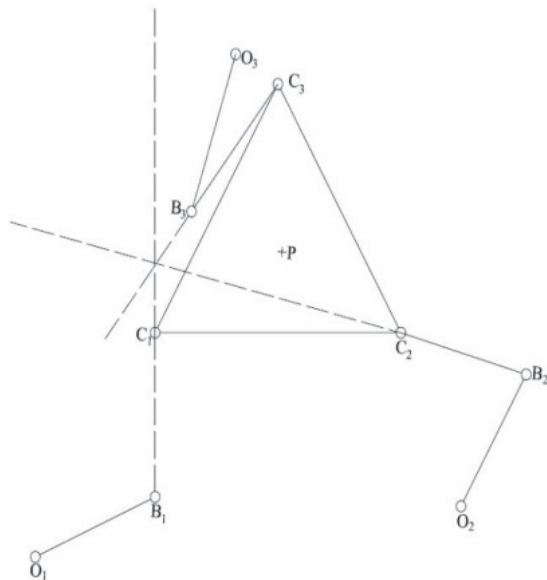
Fig. 5 Type II singularity for actuation 2
