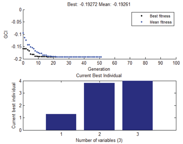
Fig. 29 Convergence of GCI for actuation 8
