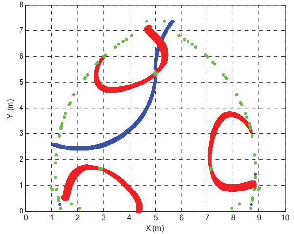
Fig. 8 Singularity loci for actuation 3
