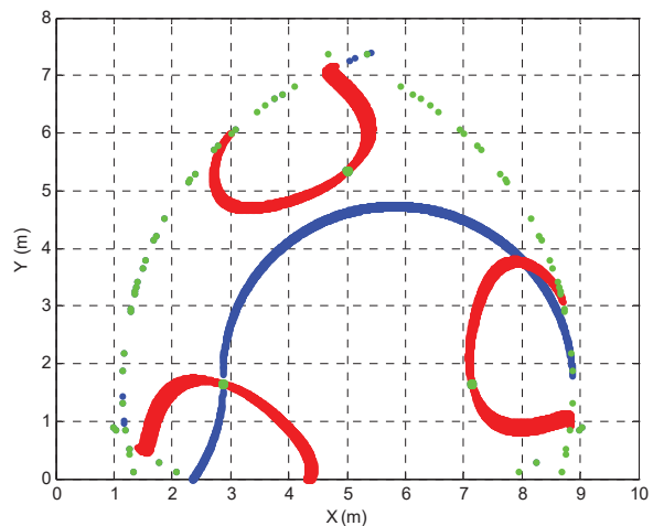
Fig. 10 Singularity loci for actuation 5
