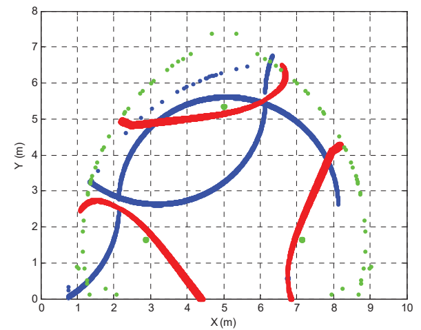
Fig. 21 Singularity loci of actuation 8
