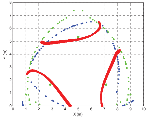
Fig. 14 Singularity loci of actuation1
