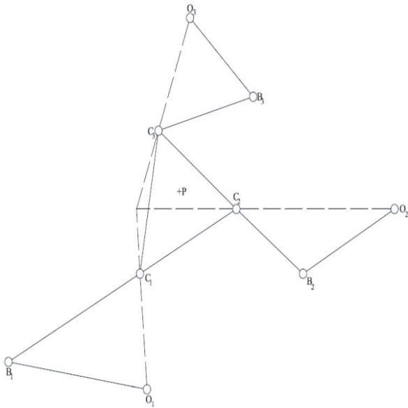
Fig. 4 Type II singularity for actuation 1
