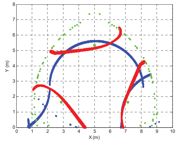
Fig. 20 Singularity loci of actuation 7
