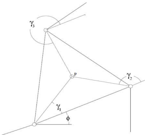
Fig. 2 End-effector description
