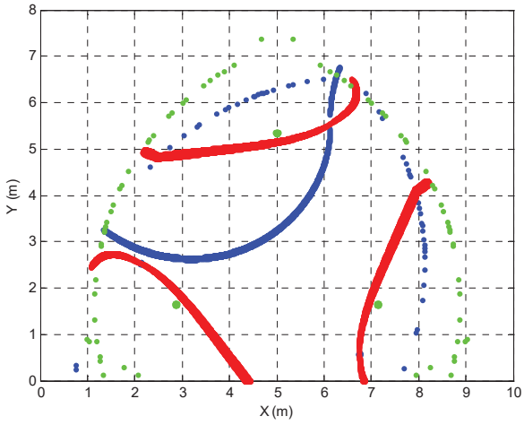
Fig. 16 Singularity loci of actuation 3
