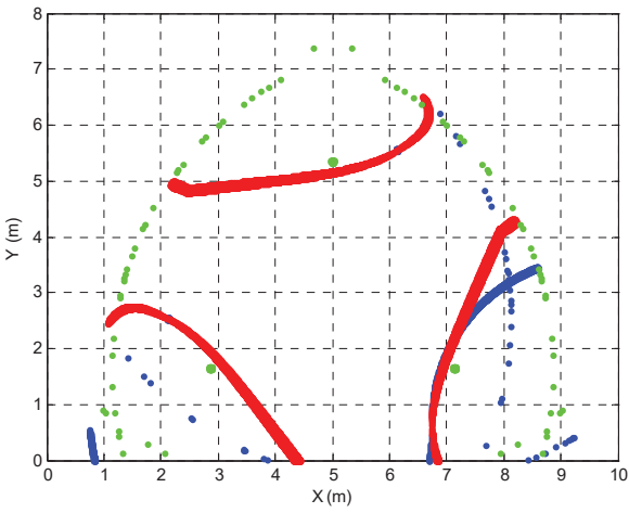
Fig. 17 Singularity loci of actuation 4
