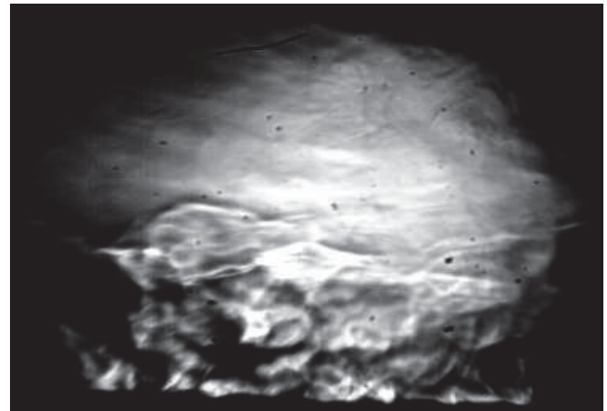
Fig. 10 Convection above the experimental sample with a Wall superheat of 30 K and an electric field of 30 kV/cm
