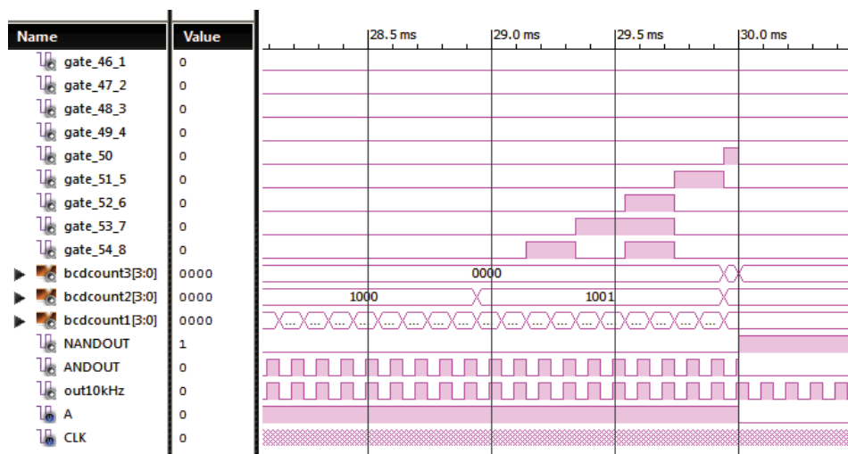
Fig. 3 (b) Simulation result at 50 Hz with encoded pulse stream 00001112
