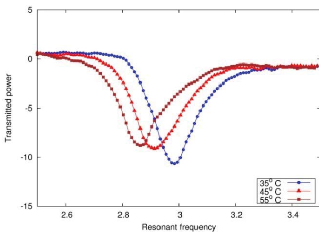
Fig. 6 Transmission curves at different temperatures of SRR when glass epoxy sample - 1 is placed on the surface
