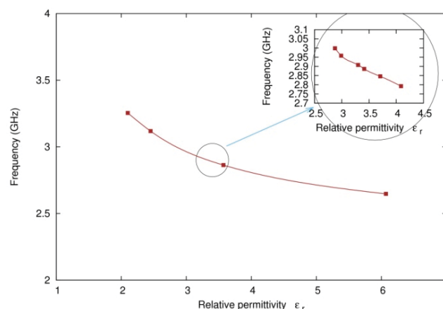
Fig. 4 Calibration graph between the resonant frequency and the relative permittivity: The inset shows the magnified view of the frequency-permittivity region for the temperature dependent permittivity region of the sample
