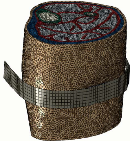
Fig. 3 Loaded FE model with the strap tightened around the lower limb
