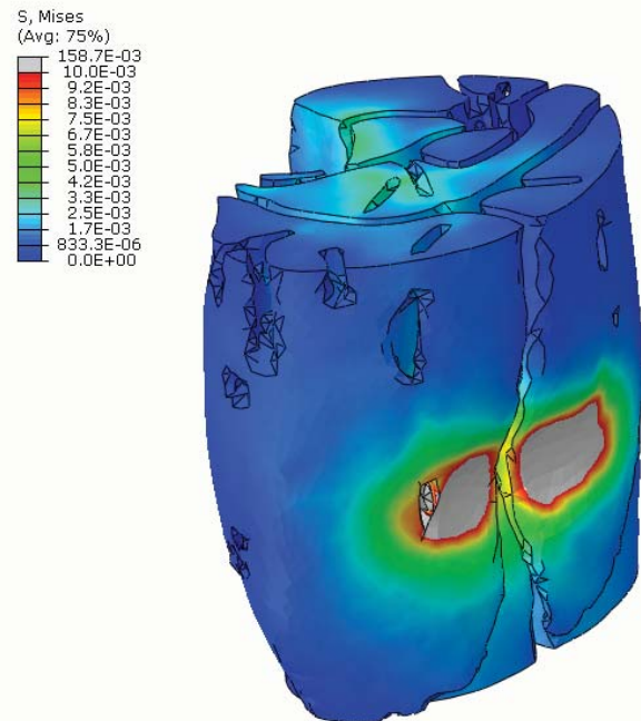
Fig. 9 Contour plot of the muscle tissue from the detailed FE model showing the von Mises effective stress
