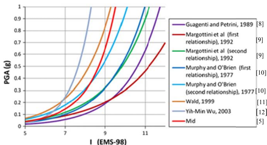
Fig. 8 Different correlations between PGA and intensity [5]
