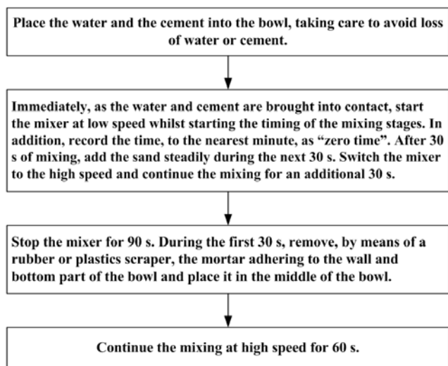
Fig. 4 Mixing procedure
