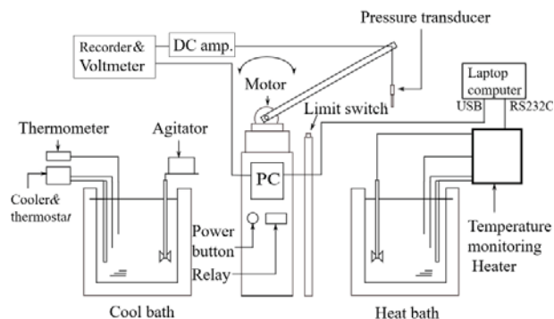
Fig. 3 Experimental apparatus
