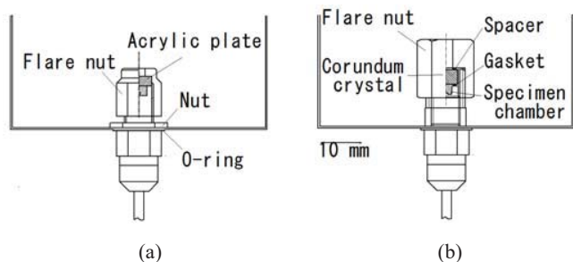
Fig. 2 Metal Berthelot tubes built in observation windows
