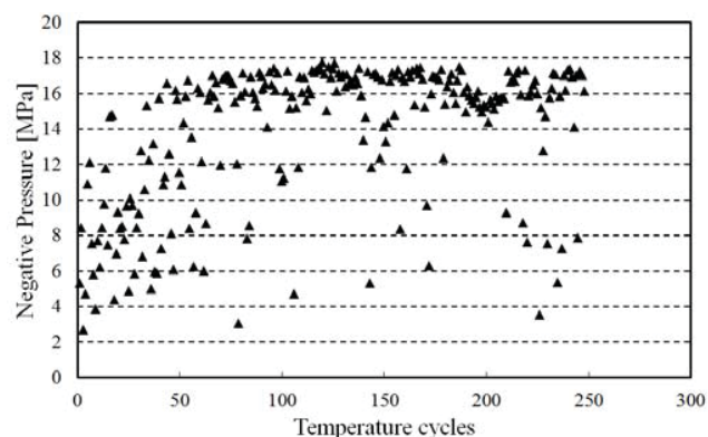
Fig. 8 Relation between negative pressure and temperature cycles for a water and methyl pyridine solution with corundum plates and Al gasket
