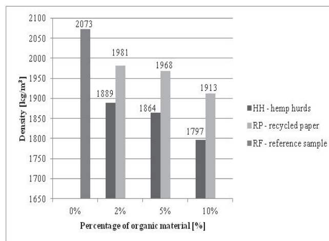
Fig. 5 Influence of organic filler content on composites density
