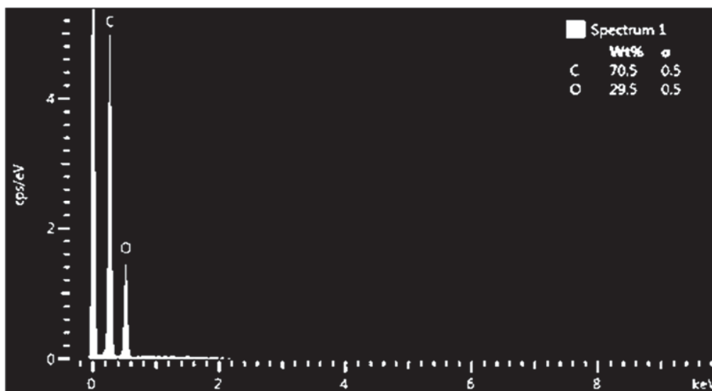
(b) Fig. 4 EDX investigation of cellulose fibers from waste paper (a); lignocellulosic hemp hurds (b)
