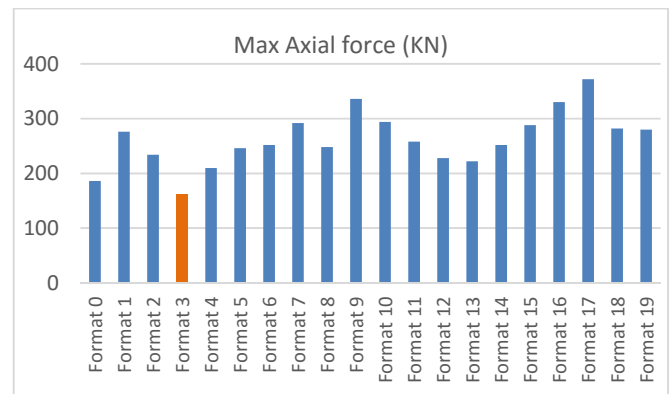
Fig. 6 Comparing the maximum axial load of the frame for each format
