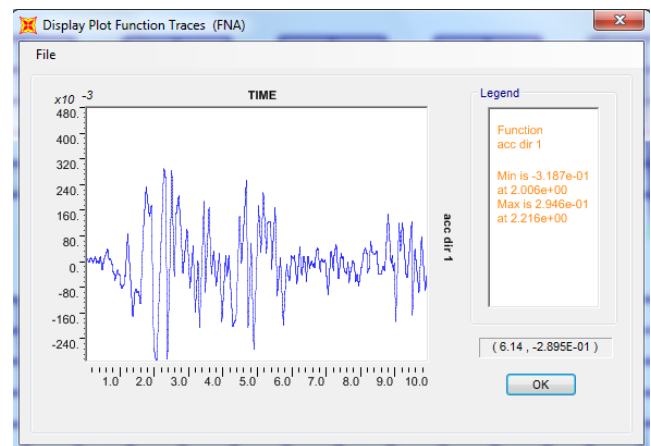
Fig. 2 Ground acceleration diagram of El Centro earthquake ground motion
