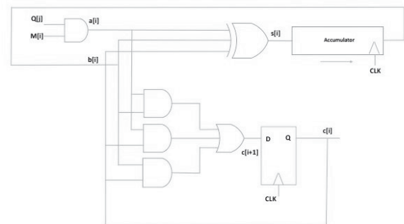
Fig. 8 Circuit for the Bit-Serial Multiplier in this Processor
