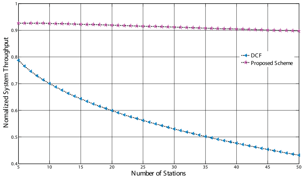
Fig. 4 Normalised system throughput of the unlicensed band
