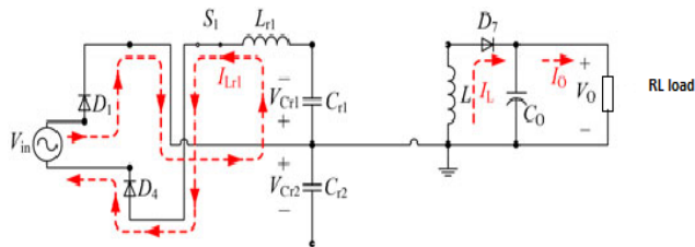
Fig.6 Equivalent Circuit Diagram of Mode 2
