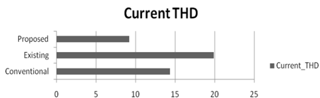
Fig. 20 Value of Current THD in the Proposed System
