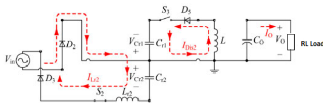
Fig. 7 Equivalent Circuit Diagram of Mode 3
