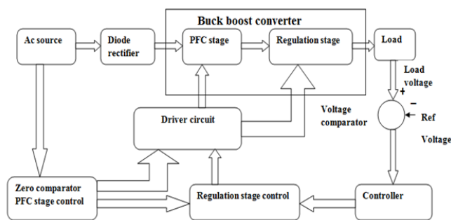
Fig. 4 Block Diagram of Proposed System
