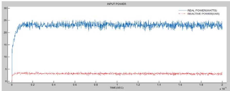
Fig.15 Waveform of input power
