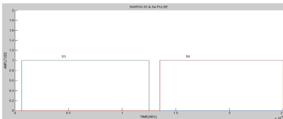
Fig. 10 Gate pulse signals for Switches S3, S4
