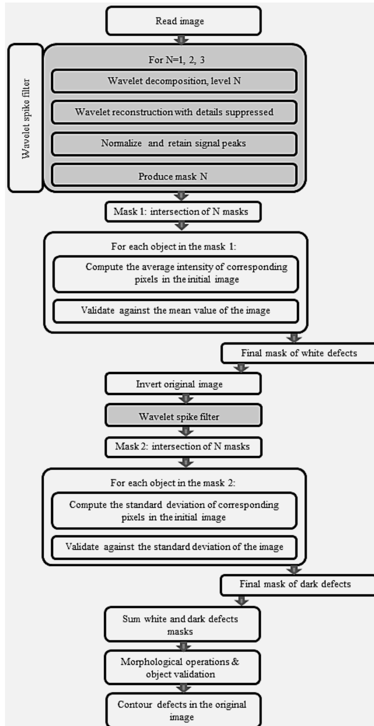
Fig. 7 Algorithm schematic sequence
