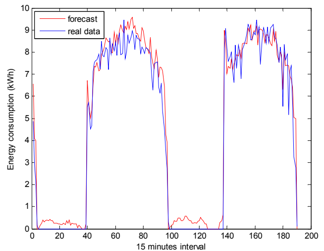
Fig. 4 Real Energy Consumption vs. Forecasting
