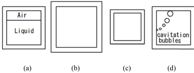
Fig. 1 Four stages of the Berthelot tube
