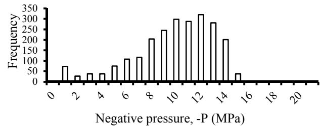
Fig. 7 Scatters in negative pressures with temperature cycles for the initial 2352 cycles for the ball of OFC having plasma treatment
