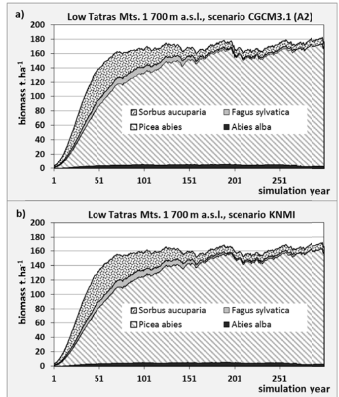
Fig. 4 The results of Forest gap model – simulation for climate change scenarios: a) CGCM3.1 A2 and b) KNMI (central part of Slovakia – 1,700 m a.s.l.)
