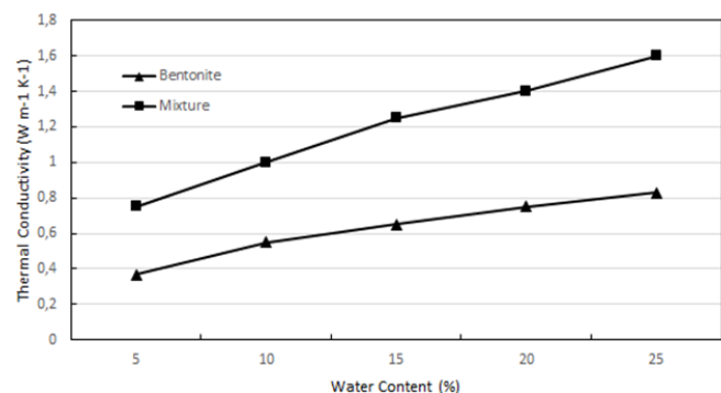
Fig. 2 Thermal conductivity of bentonite and B/S mixture, Assessment of a thermal analysis is an effective parameter for the near field analysis of buffer materials
