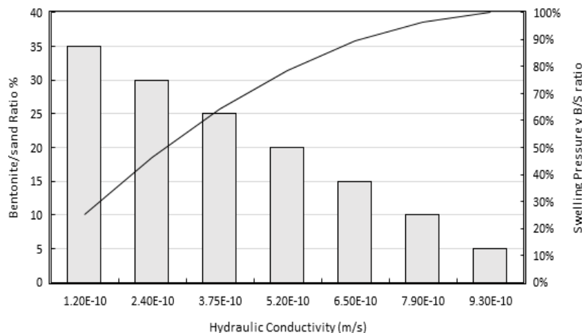
Fig. 1 Hydraulic conductivity of various B/S mixtures
