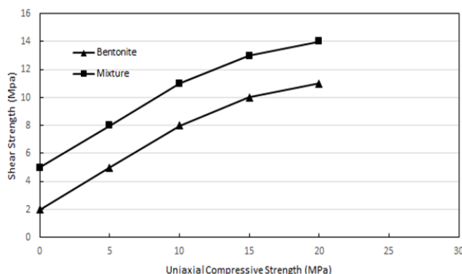
Fig. 3 Uniaxial compressive strength versus shear strength
