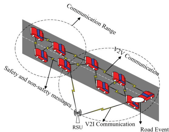
Fig. 1 VANET architecture represents V2V and V2I communication
