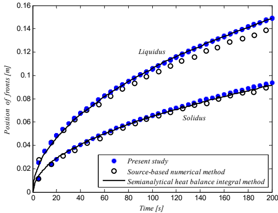
Fig. 3 Solidification of a binary Al-4,5%-Cu alloy
