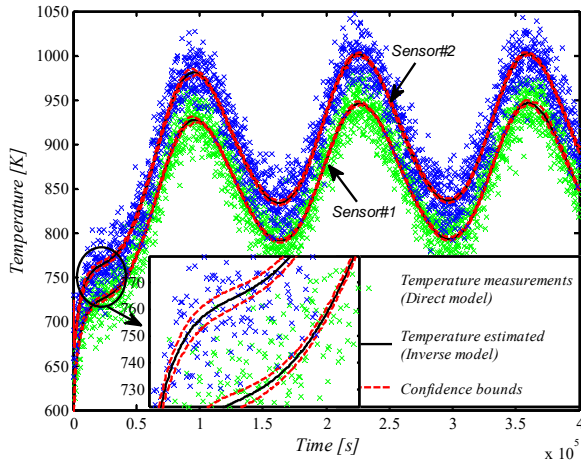
Fig. 8 Measured and inverse temperature (Sensor#1 and Sensor#2, \sigma=2\% T_{max} )
