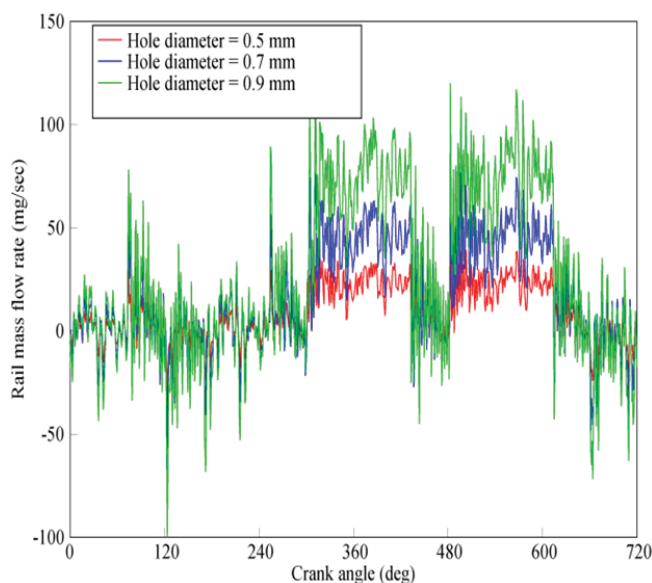
Fig. 10 Trends of rail mass flow rate with injector hole diameter
