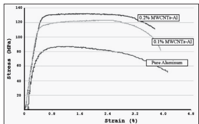
Fig. 3 Engineering tensile curves of the tested materials
