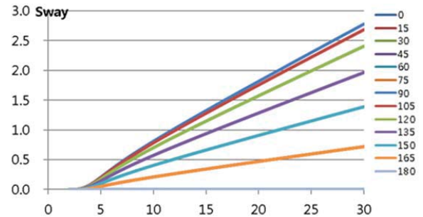
Fig. 4 Sway RAO of proposed duct
