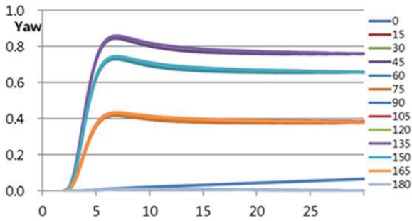
Fig. 8 Yaw RAO of proposed duct
