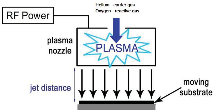
Fig. 2 Schematic diagram of atmospheric pressure plasma system [4]
