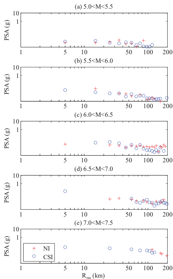
Fig. 4 Distribution of the ground motion parameters with respect to the distance at different distance-magnitude intervals for SA at 2.0 sec. “+” signs represent NI region and “o” signs denote CSI region
