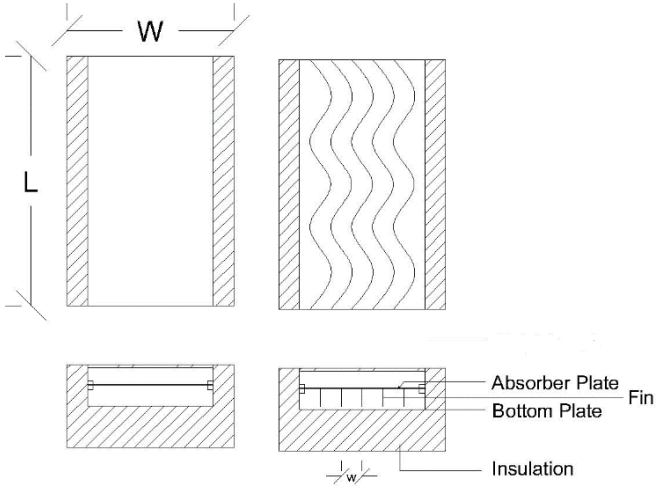
Fig. 1 Solar air heater with wavy fin absorber
