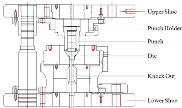
(c) Cold sizing forging mold
