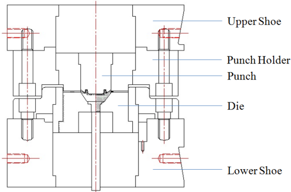
(a) Hot forging mold
