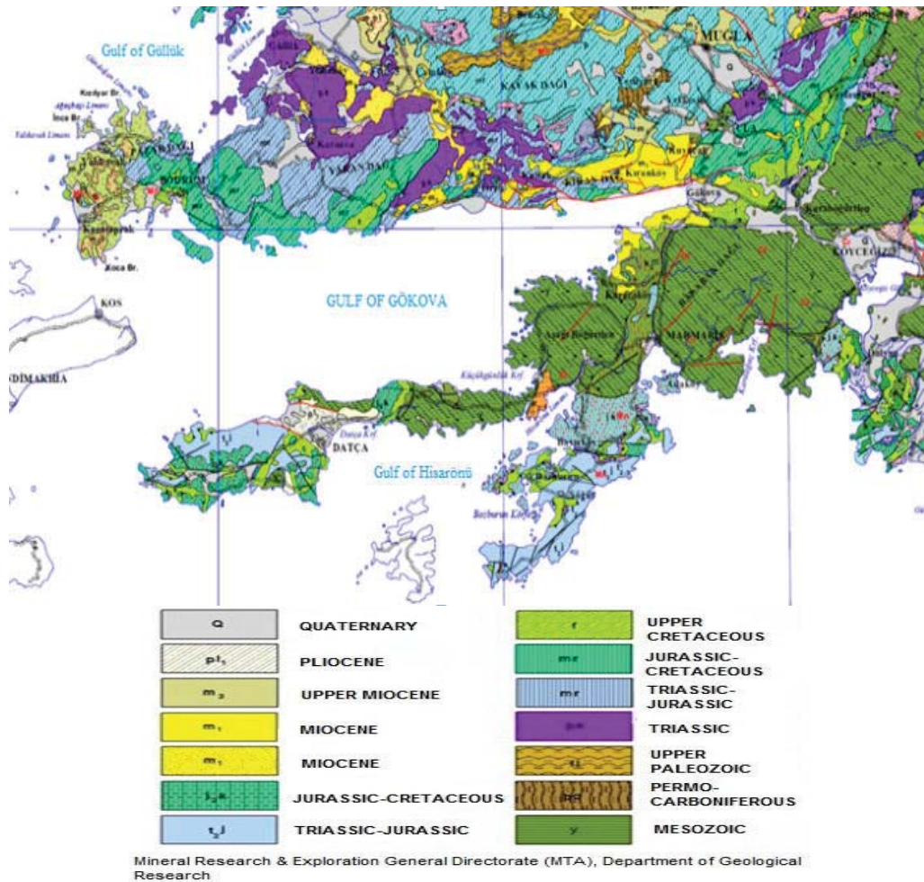
Fig. 2 Geological map of Gökova and Hisarönü region [3]
