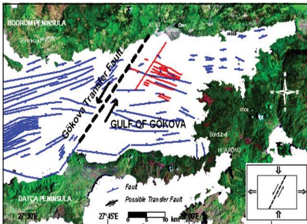
Fig. 3 Fault map of Gökova Gulf (modified from [9])
